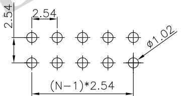
RECOMMEND PCB LAYOUT(TOLERANCE=±0.05)
