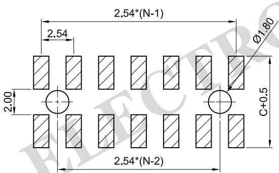
RECOMMEND P.C.B BOARD HOLE LAYOUT (TOLERANCE=±0.05)
