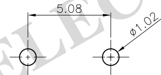
RECOMMEND PCB LAYOUT
