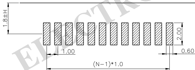
RECOMMEND PCB LAYOUT (TOLERANCE=±0.05)
