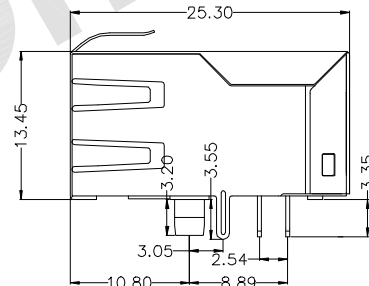
RIGHT SIDE
