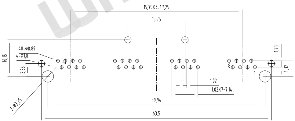
PC Board Layout Component Side View
