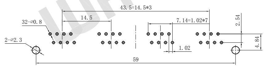
PC Board Layout Component Side Shown
