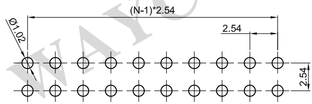
RECOMMEND PCB LAYOUT (TOLERANCE=±0.05)
