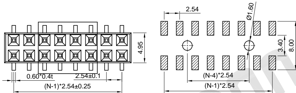
Recommend PCB layout (Tolerance:±0.05)
