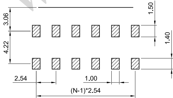
RECOMMEND PCB LAYOUT (TOLERANCE= \pm 0.05 )
