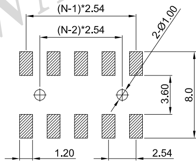
RECOMMEND PCB LAYOUT (TOLERANCE=±0.05)
