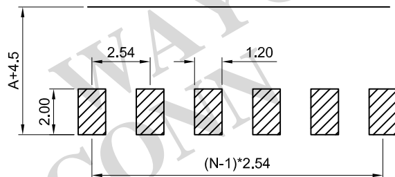
RECOMMEND PCB LAYOUT (TOLERANCE=±0.05)
