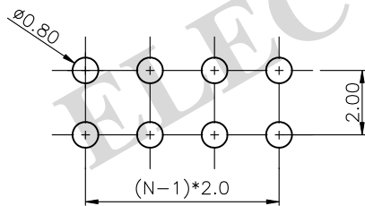
Recommended PCB Layout (Tolerance=±0.05mm)
