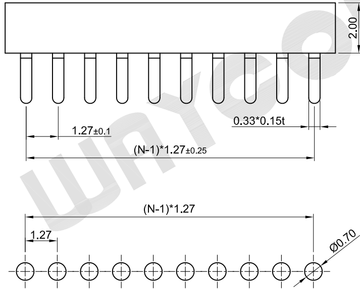
RECOMMEND PCB LAYOUT
