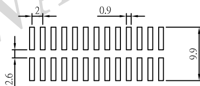
Recommended PCB Layout (PCB TOLERANCE ±0.1)
