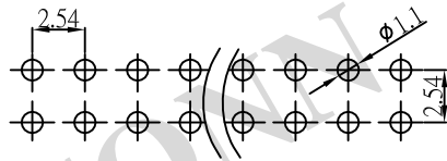
Recommended PCB Layout (PCB TOLERANCE ±0.1)
