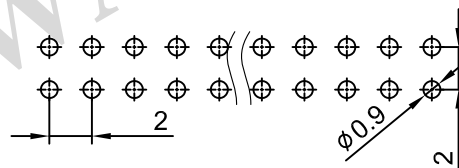
Recommended PCB Layout (PCB TOLERANCE ±0.1)
