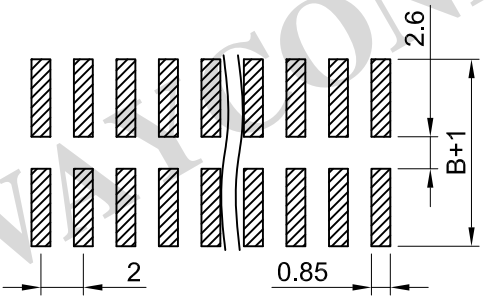
Recommended PCB Layout (PCB TOLERANCE ±0.1)
