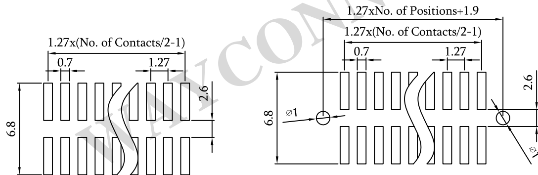
Recommended PCB Layout (PCB TOLERANCE ±0.1)
