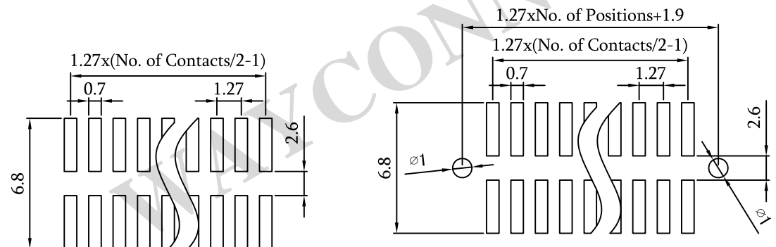
Recommended PCB Layout (PCB TOLERANCE ±0.1)
